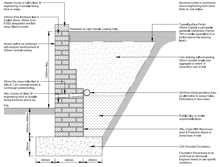
RETAINING WALL TYPE C2 (1300mm max. retained height - Pedestrian & Light Vehicle Loading Only).
