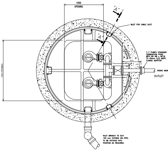
SECTIONAL PLAN VIEW 'B'-'B'
