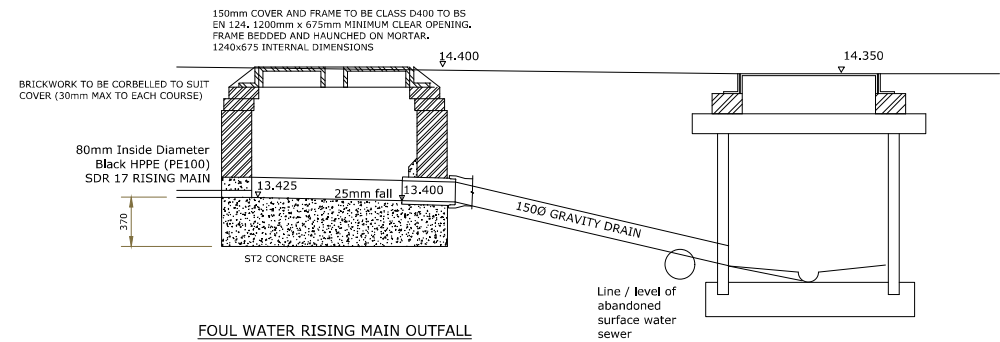
SECTIONAL PLAN ON FOUL WATER RISING MAIN OUTFALL CHAMBER
