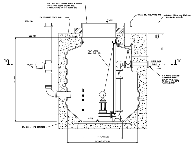
SECTIONAL ELEVATION ON OUTLET CENTRE LINE FOUL PUMPING STATION
