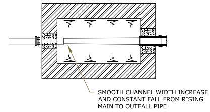
SECTIONAL PLAN ON FOUL WATER RISING MAIN OUTFALL CHAMBER
