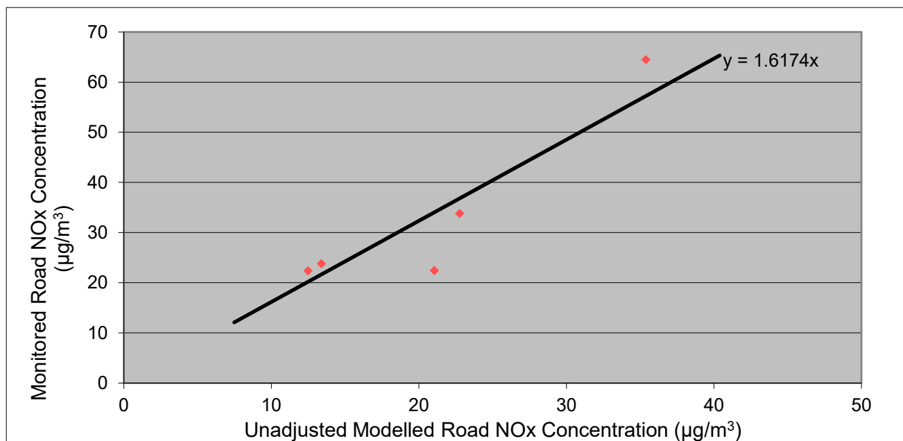
Plate 5-1 - Comparison of Monitored Road-NO x with Unadjusted Modelled Road-NO x
